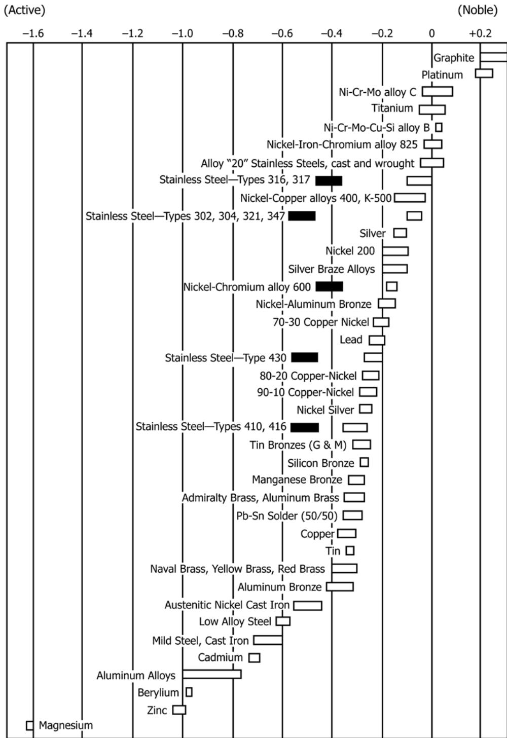
FIG. 1 Galvanic Series of Various Metals in Flowing Seawater at 2.4 m/s to 4.0 m/s for 5 to 15 Days at 5 °C to 30 °C (Redrawn from Original) (see Footnote 5)
